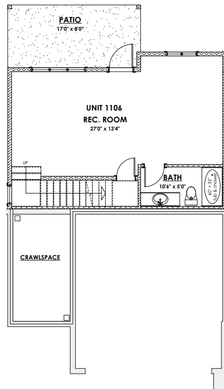
LOWER FLOOR 518 SQ FT
