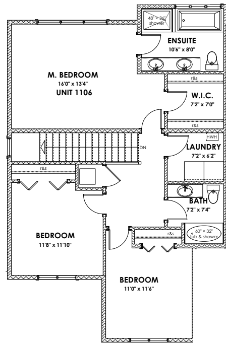
UPPER FLOOR 963 SQ FT
