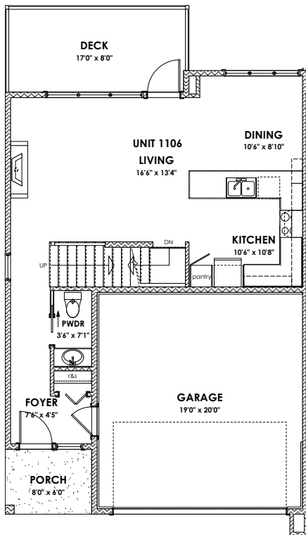
MAIN FLOOR 644 SQ FT
